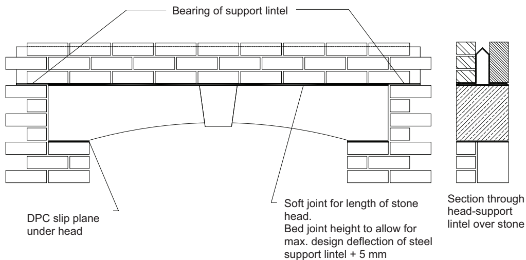
PORCH LINTEL—FRONT ELEVATION
