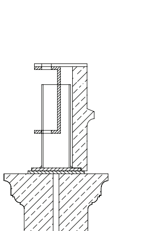
SECTION DETAIL C-C
