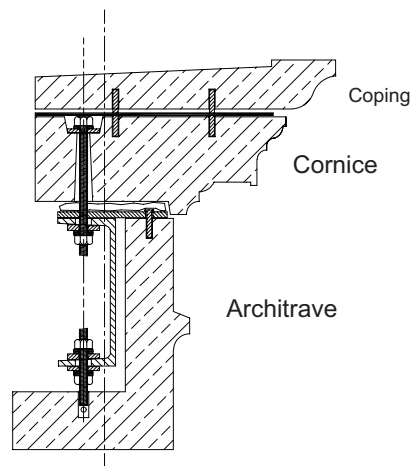
SECTION DETAIL B-B
